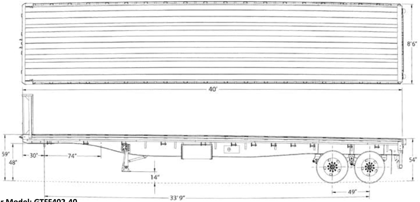
Trailer Model: GTFF402-40
