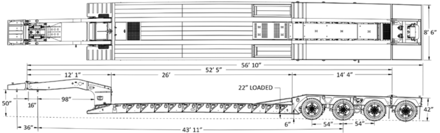
Trailer Model: GTBN553-54-26-HGG Weight: Apx. : 29171.92 ± lbs
